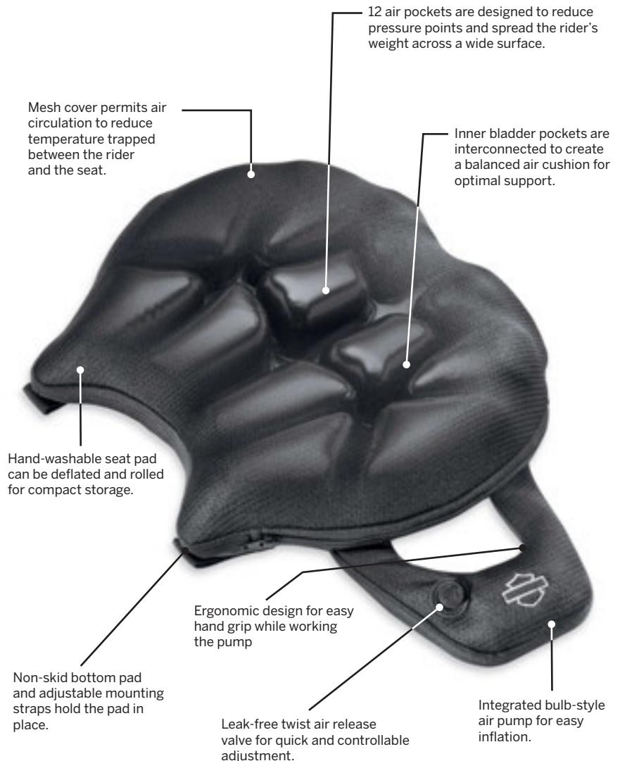
A. ROAD ZEPPELIN SEAT PAD
